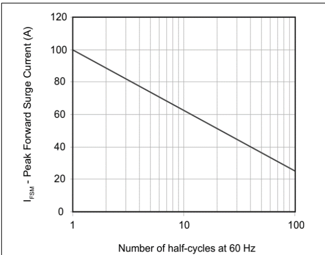
Figure 4. Maximum non-repetitive surge current
