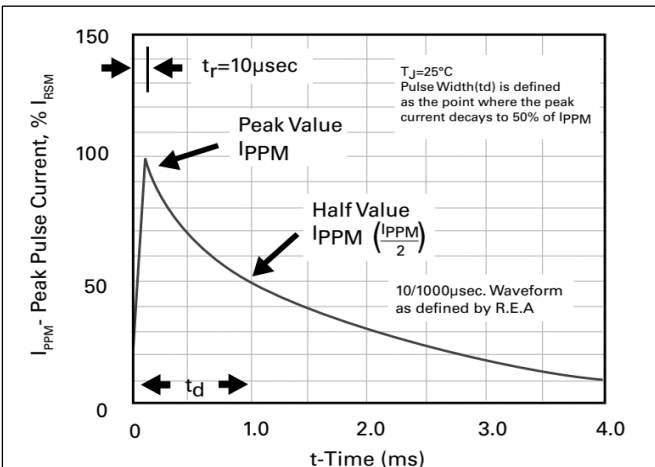
Figure 2. Pulse waveform
